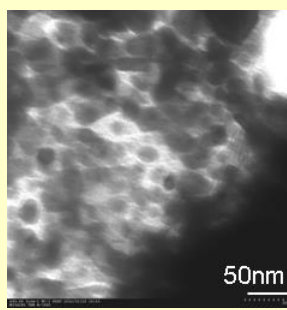
FeCo alloy particles 10~20nm
