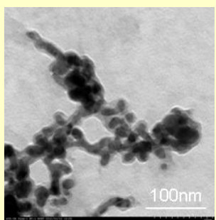
Ni nanoparticles 20nm
